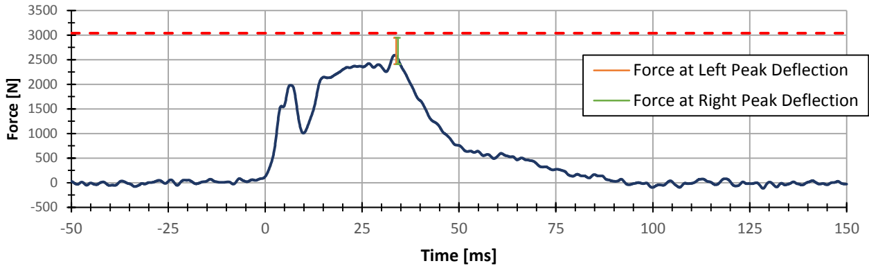
Probe Force
