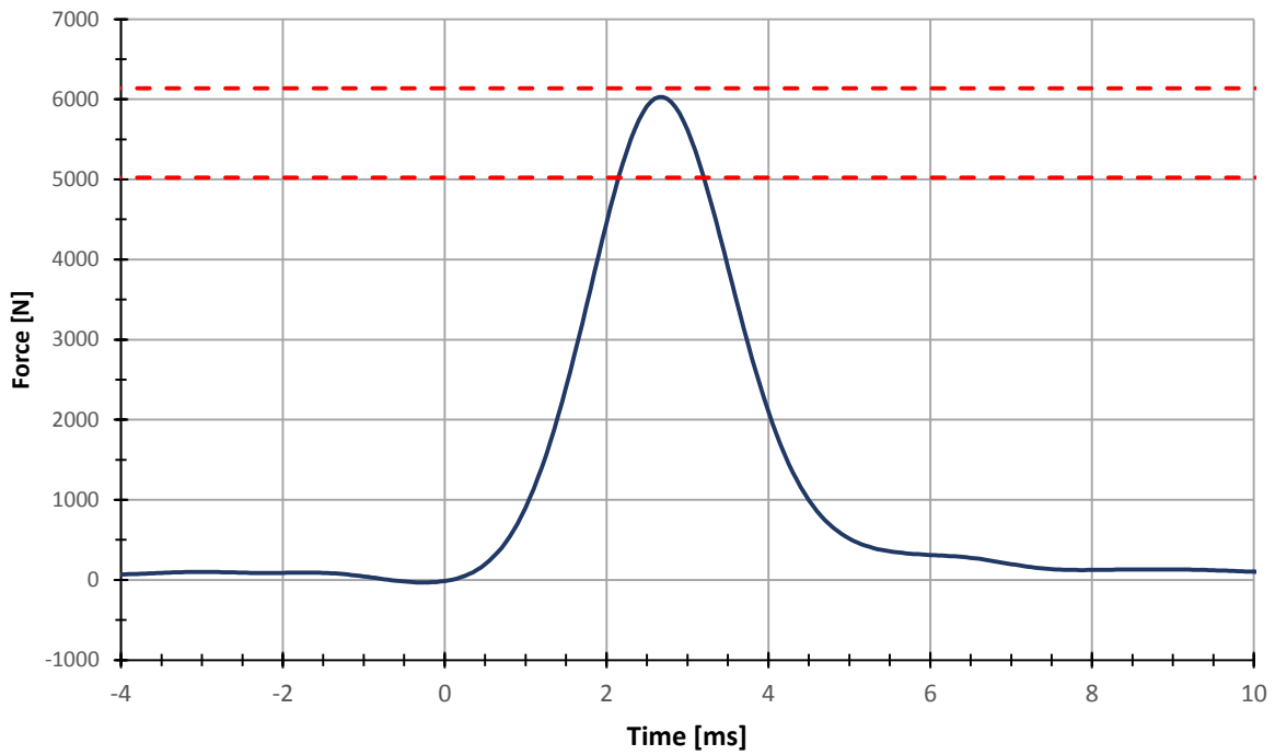
Probe Force
