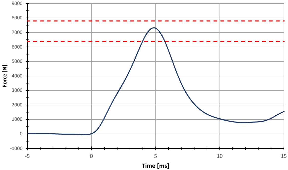
Probe Force
