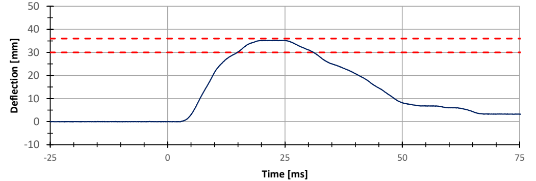
Abdomen Rib 2 Deflection
