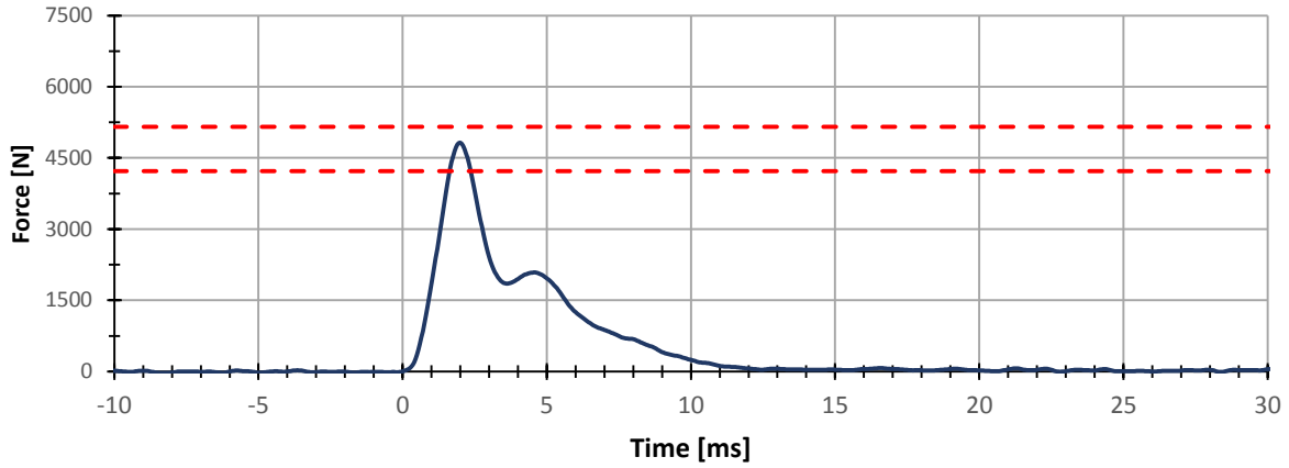
Probe Force
