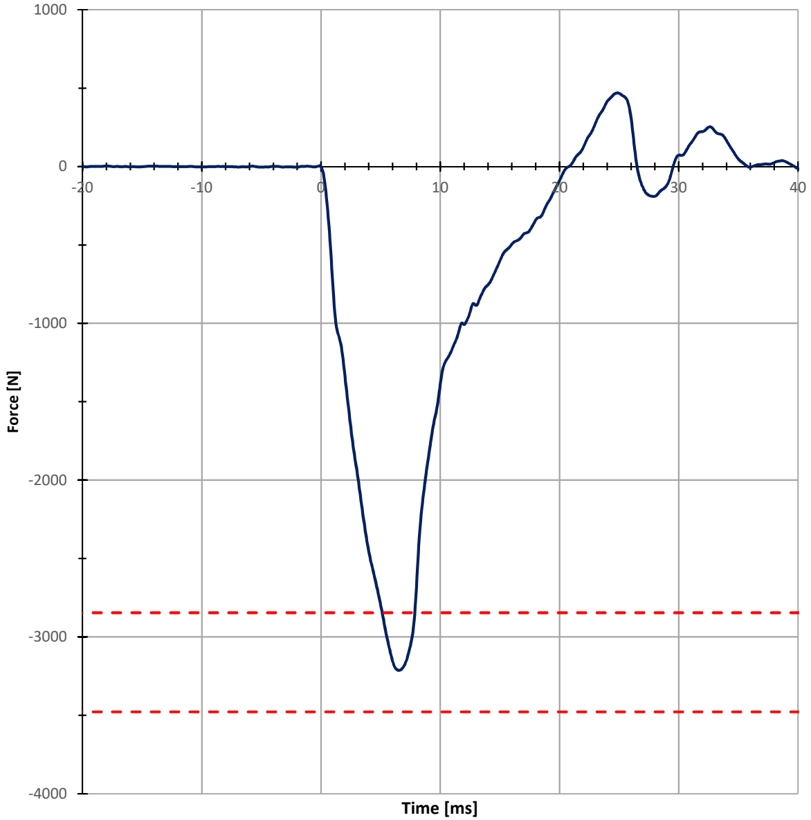
Lower Tibia Z-axis Force
