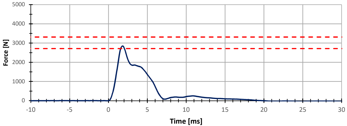
Femur Force, Fz
