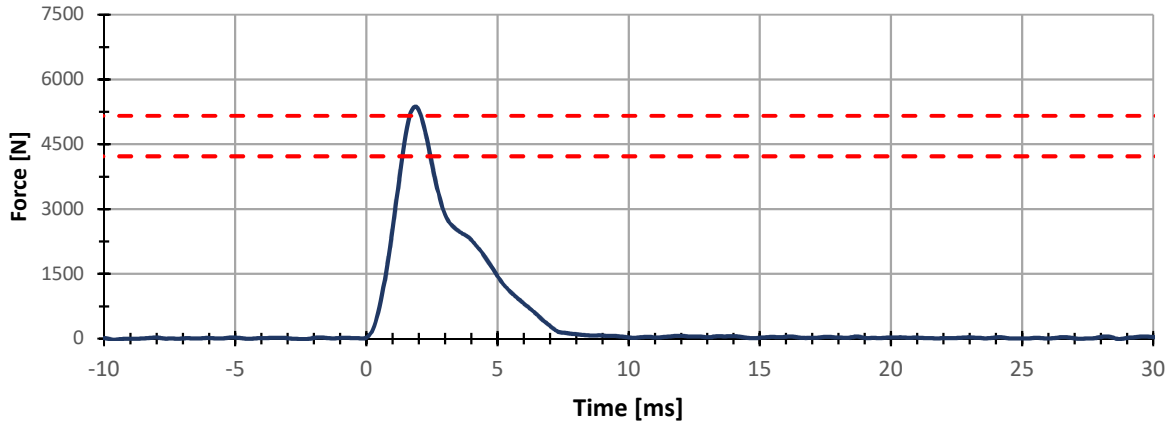
Probe Force
