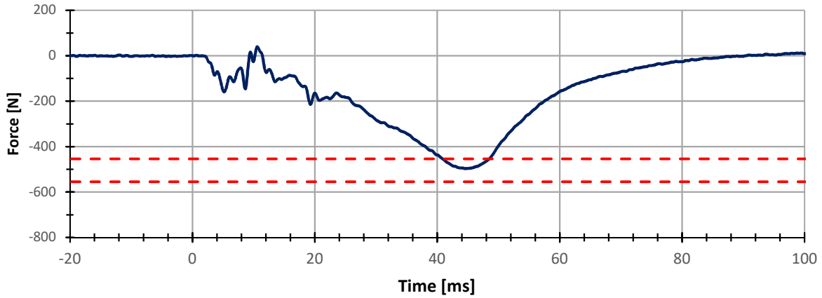
Lower Tibia Z-axis Force
