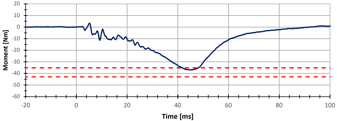
Ankle Resistive Moment
